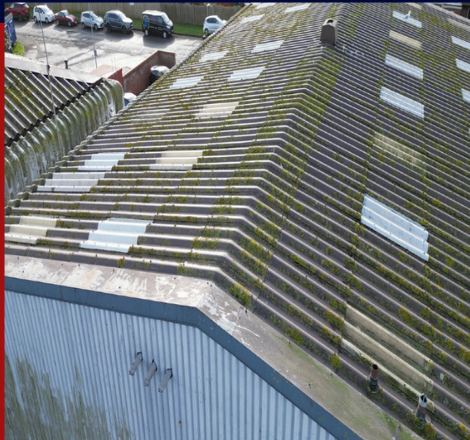
EXISTING ROOF WITH ASBESTOS CEMENT SHEETING
